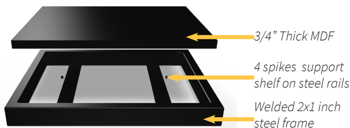
Optional IS Isolation Shelf
