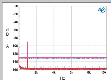
Fig.5 Bryston BDA-3, spectrum with noise and spurs of dithered 1kHz tone at -90dBFS with: 16-bit data (left channel cyan, right magenta), 24-bit data (left blue, right red) (20dB/vertical div.).
