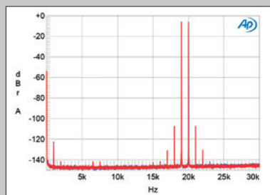
Fig.9 Bryston BDA-3 with upsampling, HF intermodulation spectrum, DC-30kHz, 19+20kHz at OdBFS into 100k ohms, 44.1kHz data (left channel blue, right red; linear frequency scale).
