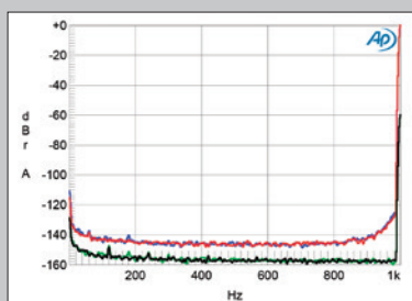
Fig.4 Bryston BDA-3, spectrum with noise and spurs of dithered 24-bit 1kHz tone at 0dBFS (left channel blue, right red) and -60dBFS (left green, right gray) (20dB/vertical div.).
