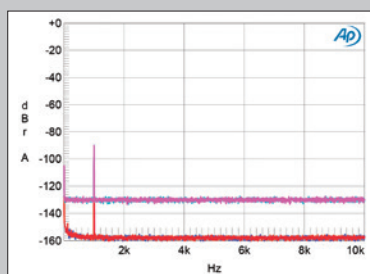
Fig.5 Bryston BDA-3, spectrum with noise and spurs of dithered 1kHz tone at -90dBFS with: 16-bit data (left channel cyan, right magenta), 24-bit data (left blue, right red) (20dB/vertical div.).
