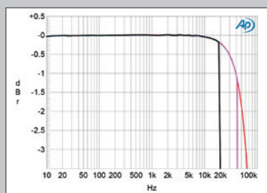
Fig.3 Bryston BDA-3, frequency response at -12dBFS into 100k ohms with data sampled at: 44.1kHz (left channel green, right gray), 96kHz (left cyan, right magenta), 192kHz (left blue, right red), 384kHz (left green, right gray) (0.5dB/vertical div.).
