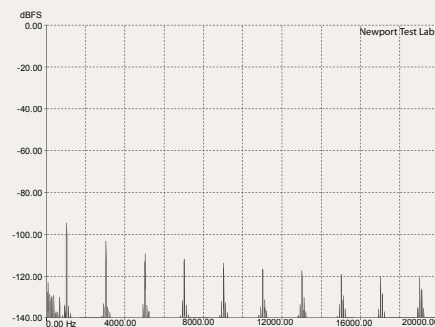
Graph 6. THD @ 1kHz @ -91.24dB recorded level. (No dither)
