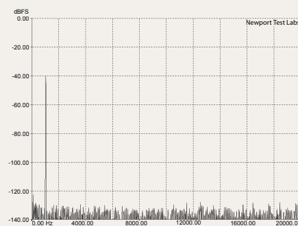
Graph 4. THD @ 1kHz @ -40dB recorded level.
