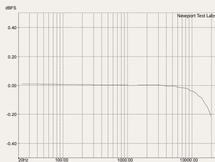
Graph 10. Frequency Response at @ 0dB recorded level.
